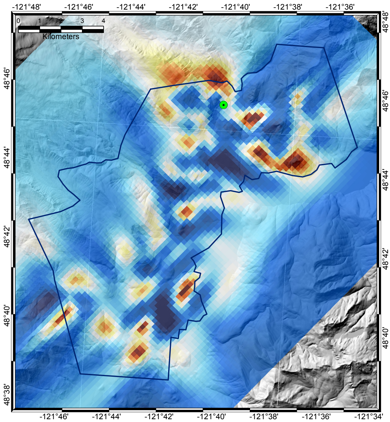
Figure 5: Depth slice at 560 m. Green dot is hot spring location.
