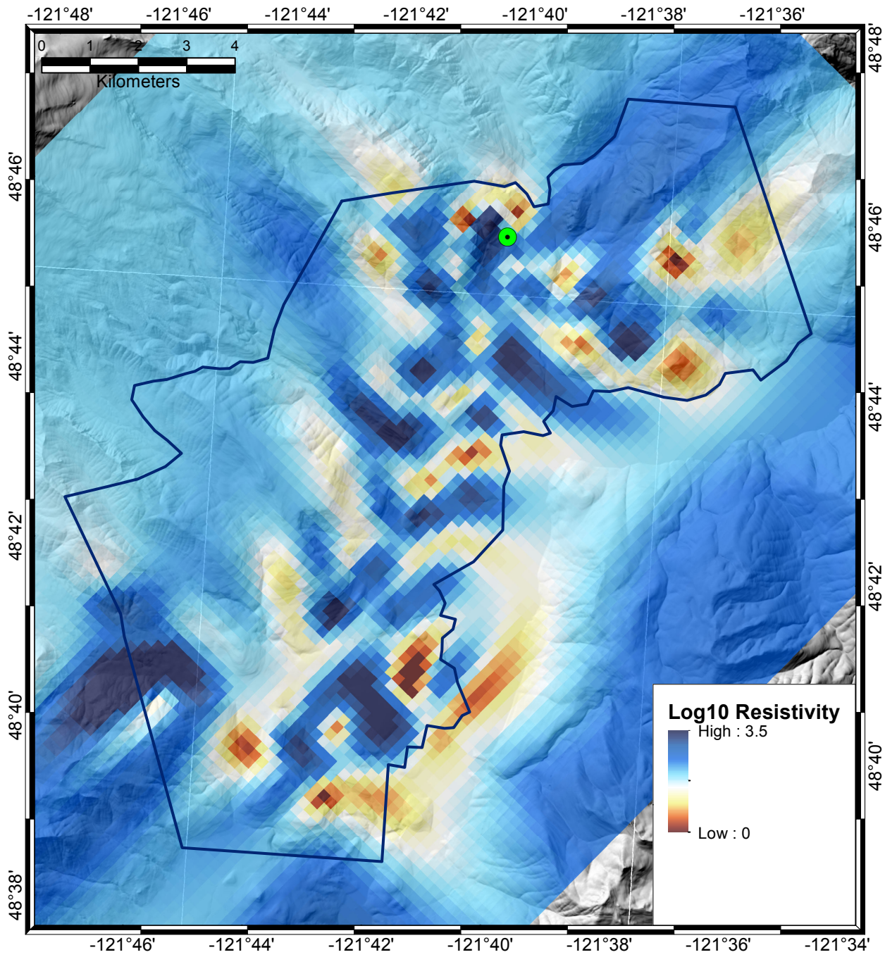
Figure 4: Depth slice at 290 m. Green dot is hot spring location.
