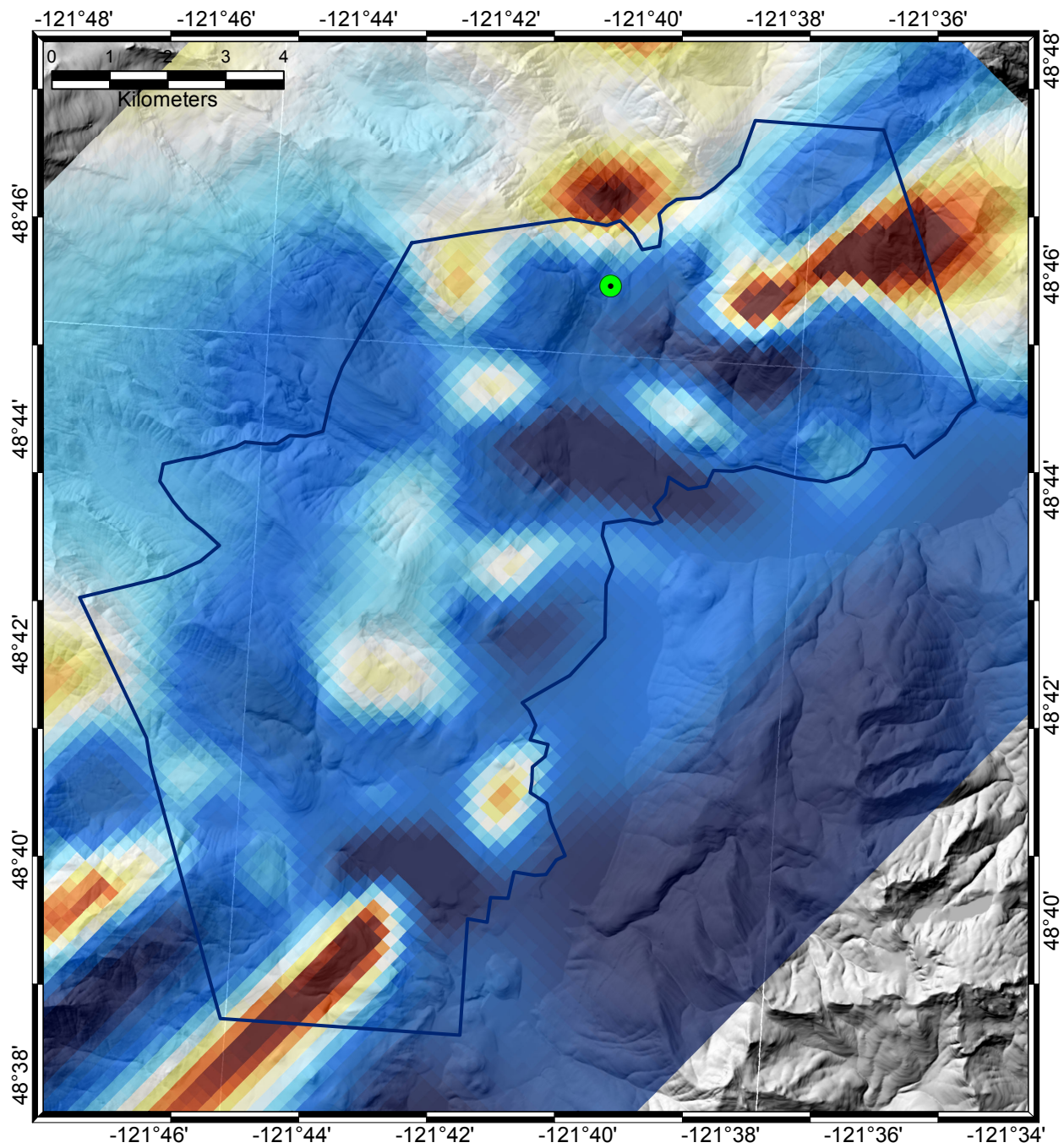
Figure 7: Depth slice at 1460 m. Green dot is hot spring location.
