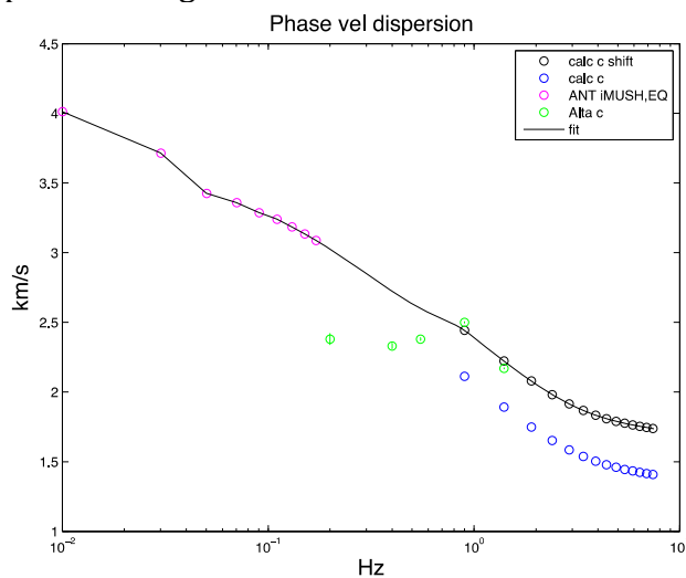
Figure 5. Dispersion curve (black line) used for 1D average shear velocity start model. Pink points are phase velocities from ambient noise tomography on iMUSH array and EQ tomography on western
