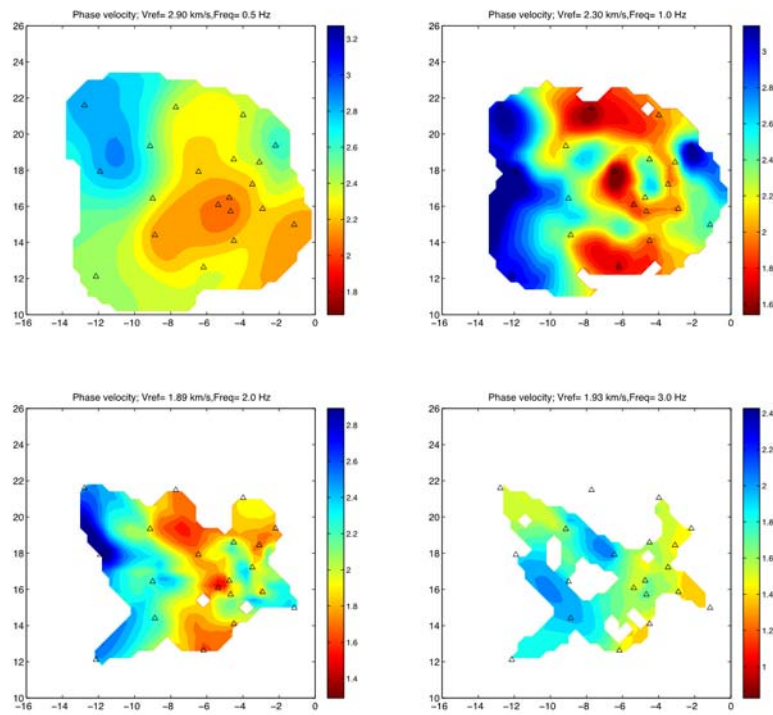
Figure 8. Phase velocity maps at four different frequencies plotted where resolution is greater than 0.
