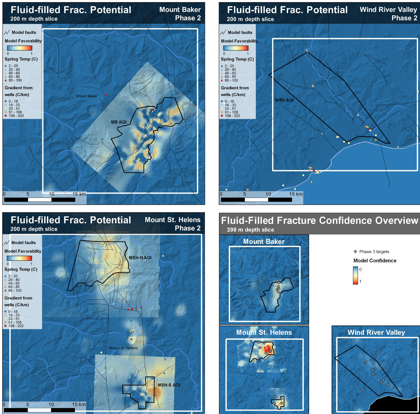
Figure 5. Phase 2 fluid-filled fracture potential at 200 m depth and overview of confidence. Data sets vary substantially between study areas and make comparisons between areas difficult. Potential models at 2 km depth are provided in Appendix I and confidence models are provided in Appendix J.
