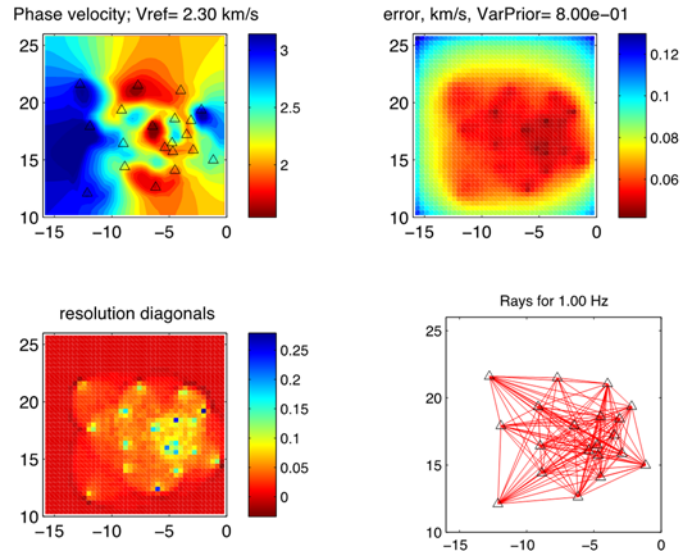
Figure 3. Top left: Inversion using finite frequency methods for phase velocity map at one 1 Hz . Top right: calculated error. Bottom left: Resolution matrix. Bottom right: Ray paths for each station pair used.
