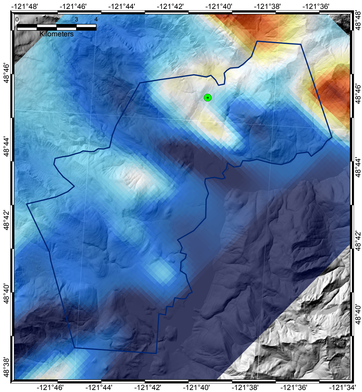
Figure 9: Depth slice at 3260 m. Green dot is hot spring location.
