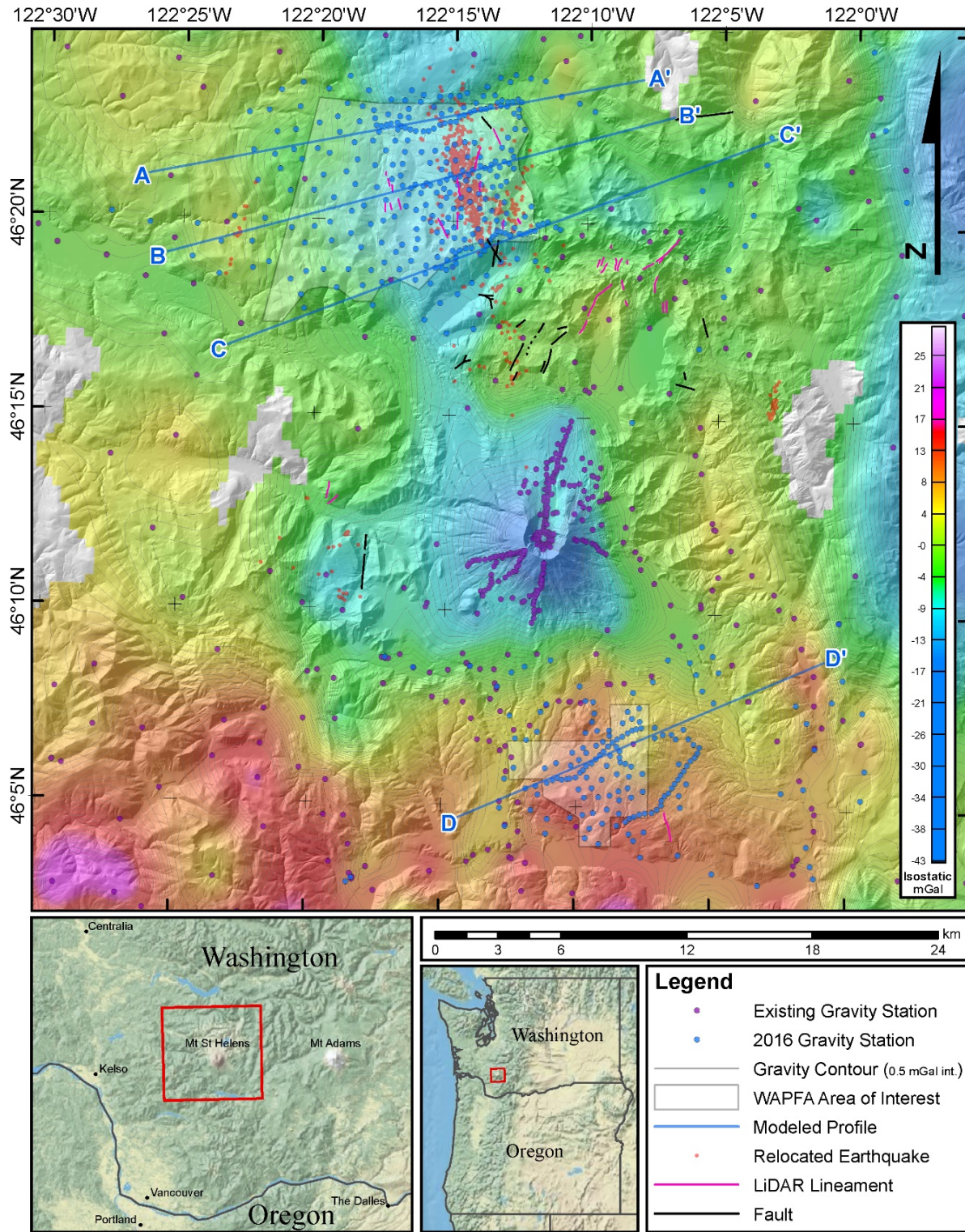
Figure 9. Isostatic gravity grid with contours, produced from stations collected during this study and pre-existing stations across Northern and Southern Areas of Interest.
