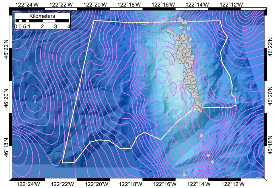
Figure 13: Resistivity depth slice at 11000 m with isostatic gravity contours (magenta lines) and earthquake locations (gray circles) within 2000 m of the depth slice.
