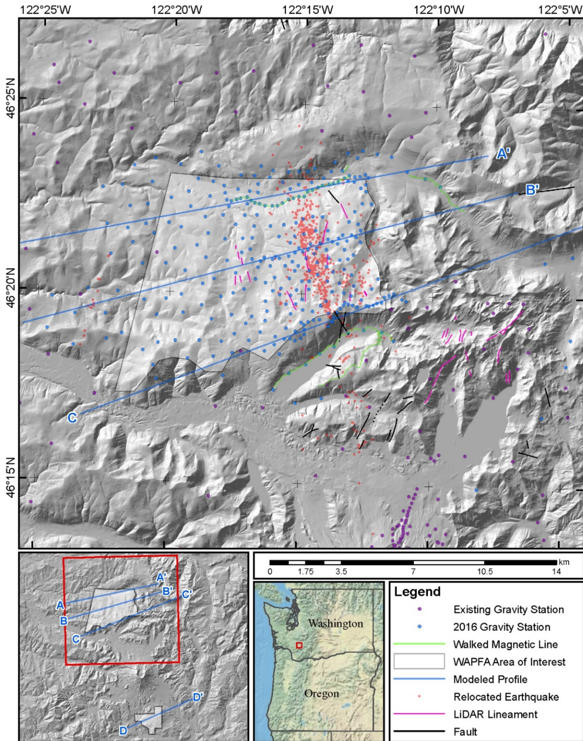
Figure 11. Location of gravity stations, walked magnetic lines, and modeled profiles within the Northern Area of Interest.
