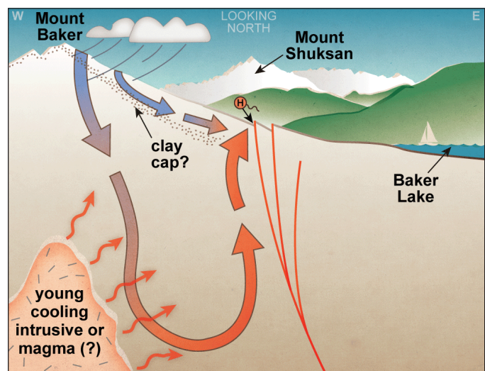
Figure 2. Updated conceptual models for Mount Baker (left), Mount St. Helens (below left), and Wind River Valley (below). Abundant Quaternary volcanism provides heat; active deformation along faults and fractures provides permeable pathways for the convection of geothermal fluids. Models are not to scale; viewing directions are provided in white at the top of each figure.
