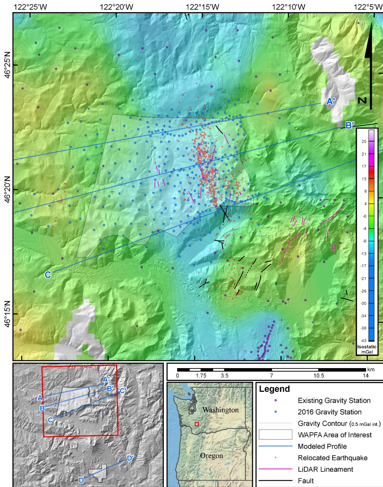
Figure 12. Isostatic gravity grid with contours, units in milligals produced from stations collected during this study and from pre-existing stations within the Northern Area of Interest.
