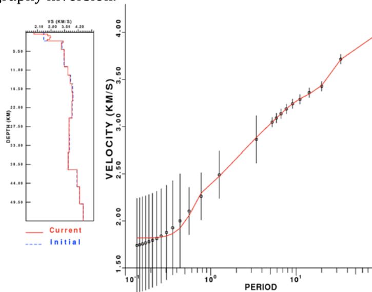
Figure 6. Left: 1D shear velocity inversion result (red) and starting model (blue). Right: the fit to the dispersion curve from slant stacking and higher period results from iMUSH and earthquake surface wave tomography (Janiszewski et al. 2016 AGU poster) used to calculate shear velocity.
