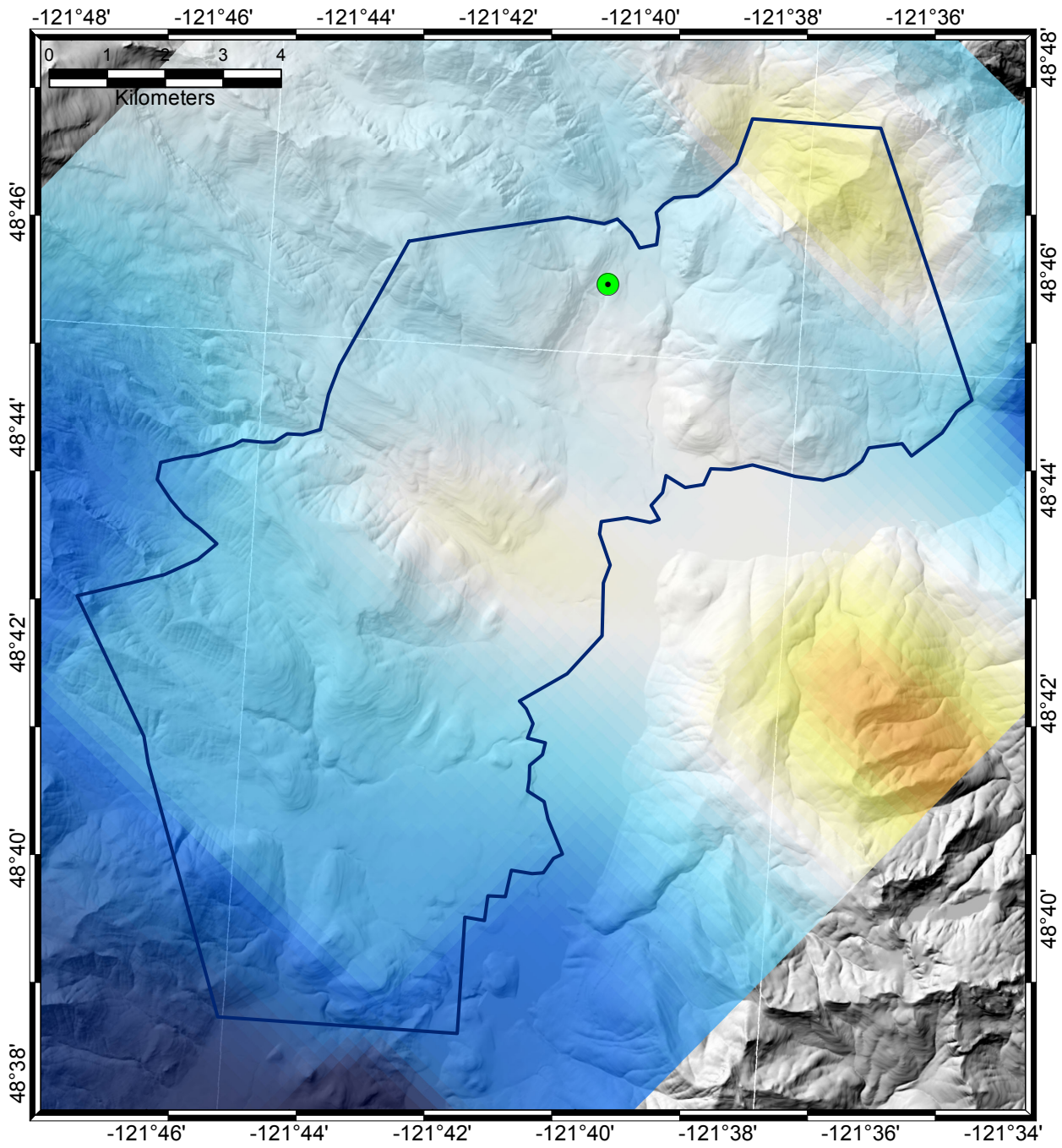
Figure 12: Depth slice at 11860 m. Green dot is hot spring location.
