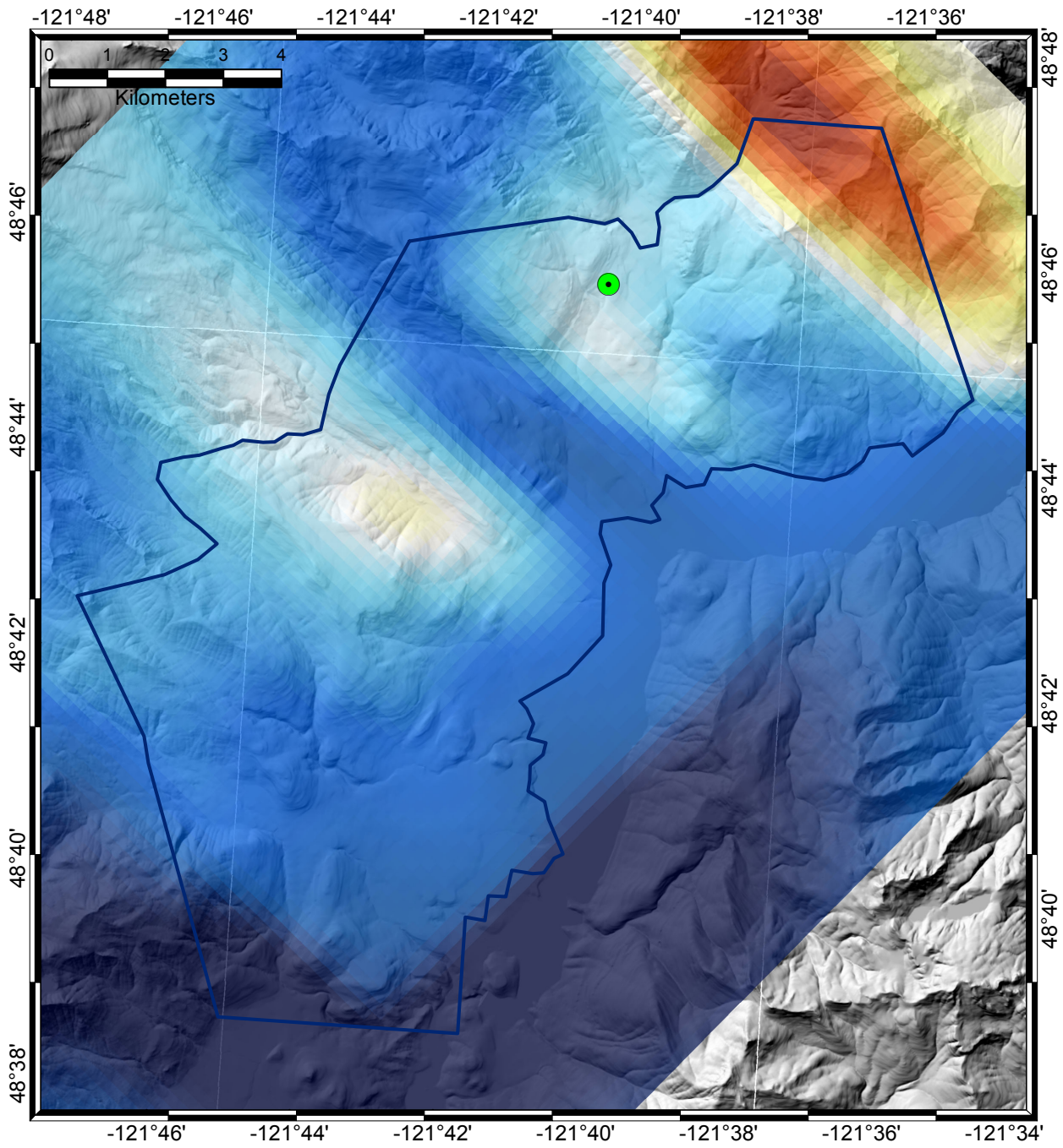
Figure 10: Depth slice at 5860 m. Green dot is hot spring location.
