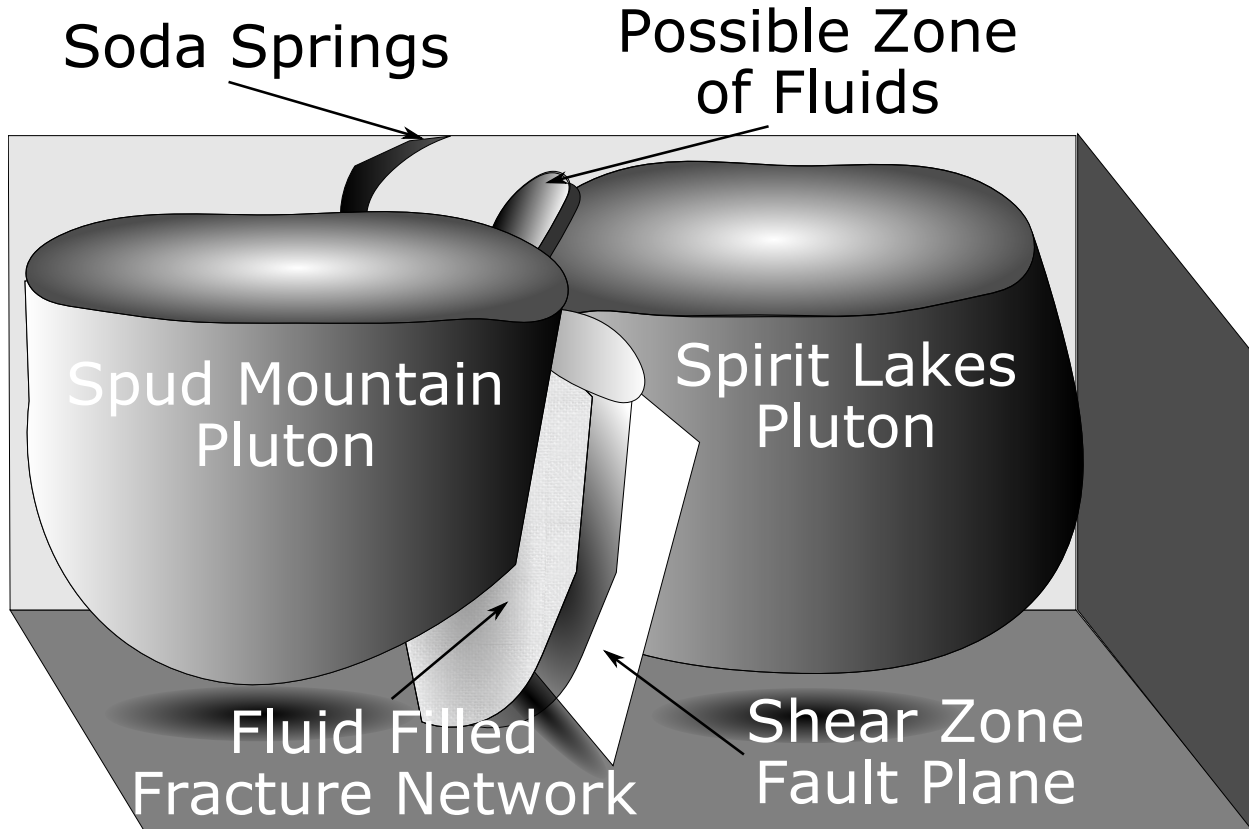
Figure 4: Schematic cartoon of geological features.
