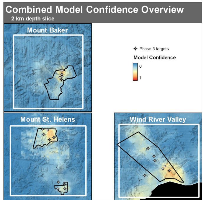
Figure 7. Phase 2 Combined favorability models at 2 km depth with overview of confidence. Full-size confidence models are provided in Appendix J.
