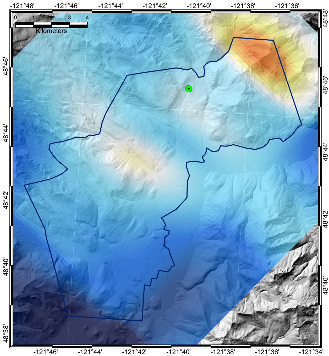
Figure 11: Depth slice at 7860 m. Green dot is hot spring location.
