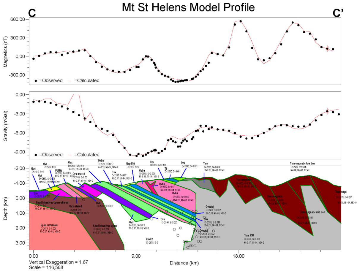
Figure 23. 2D Potential field model along profile CC' in the Mount St. Helens study area. Panels show observed (black circles) and model (red line) anomalies for magnetic (top) and gravity (middle) fields, and potential field model with individual model bodies colored by rock unit (bottom). Open circles are earthquake hypocenters from the PNSN catalog. Profile location shown on Figure 8.
