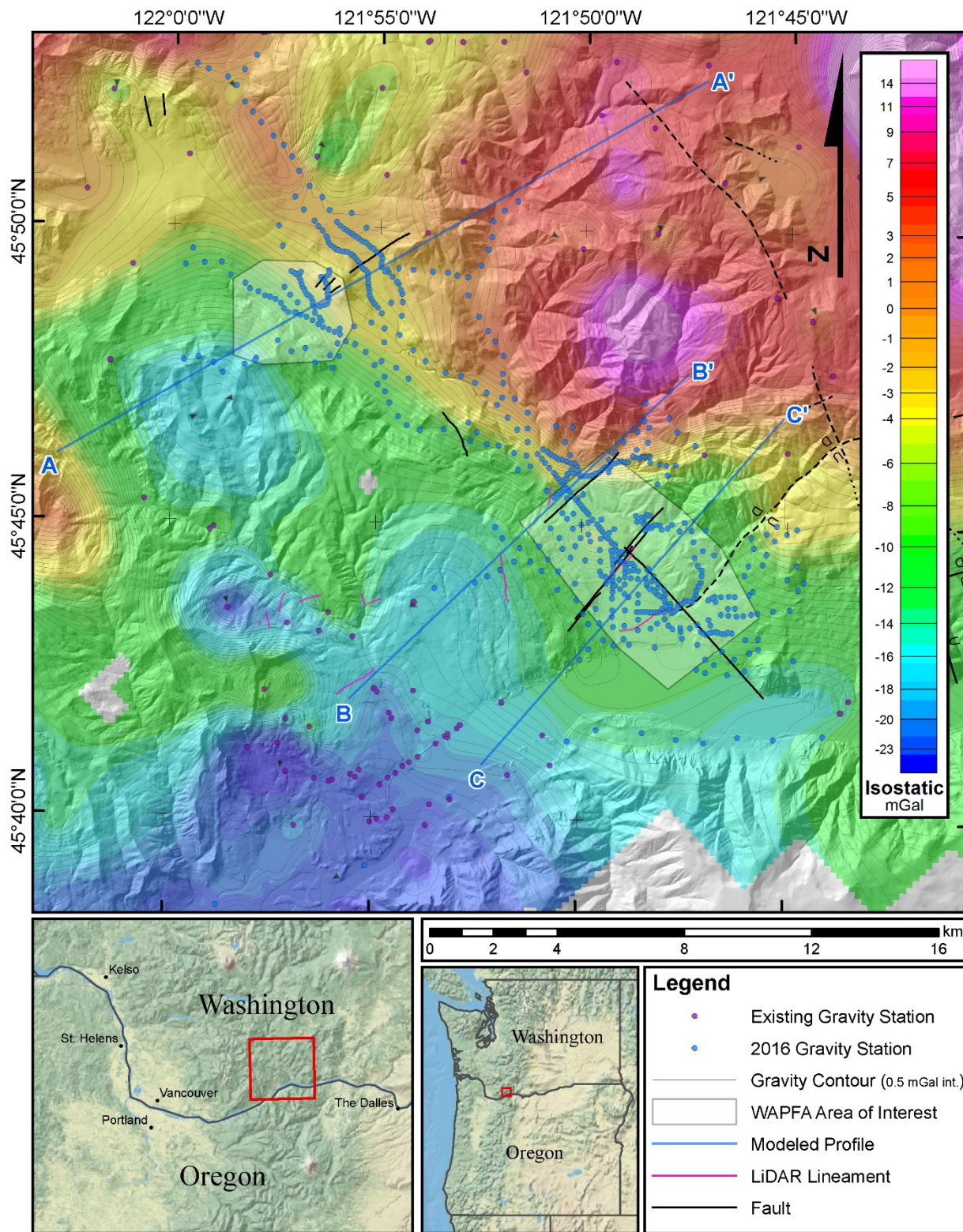
Figure 2. Isostatic gravity grid with contours, units in milligals produced from stations collected during this study and pre-existing stations.
