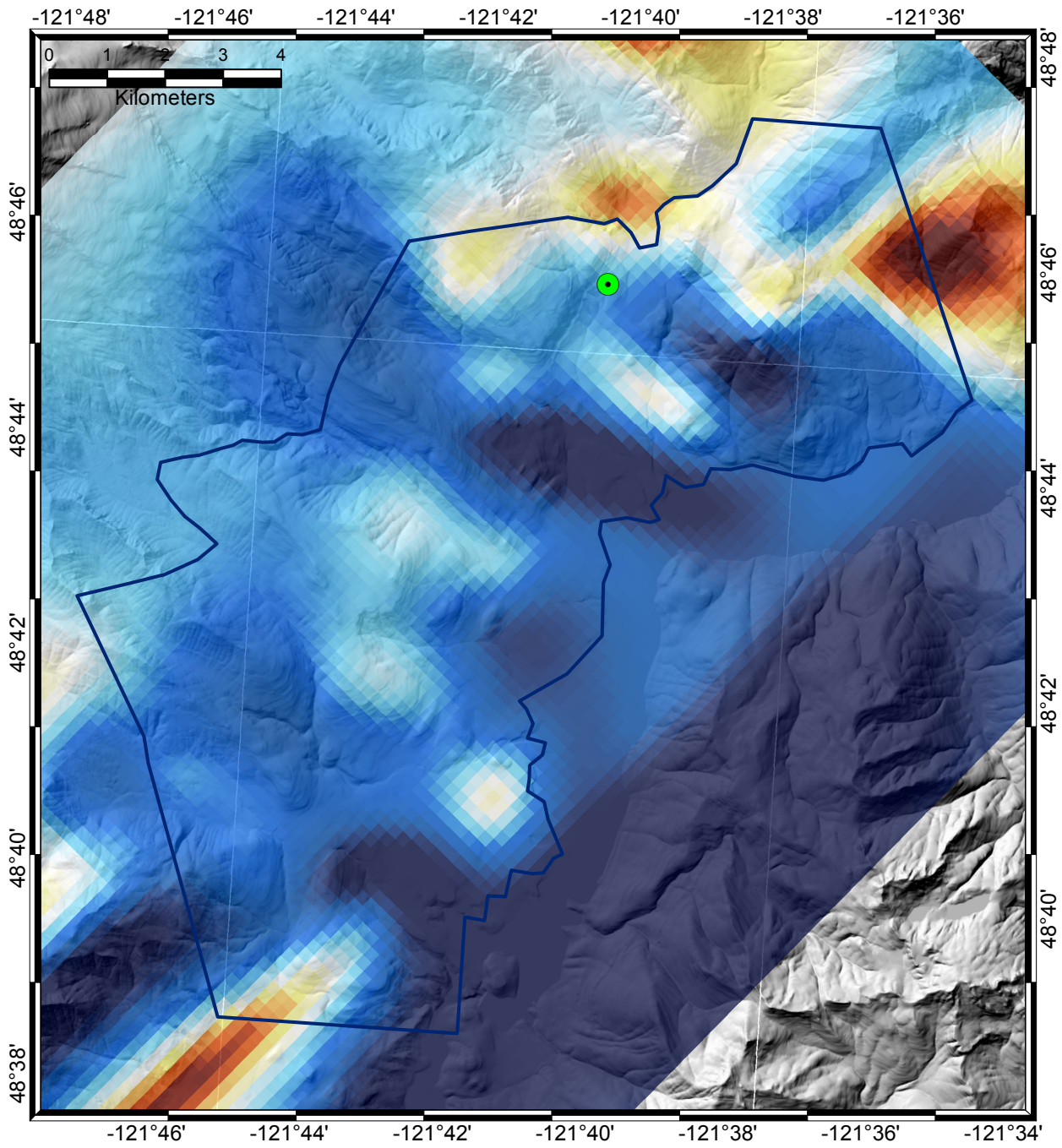
Figure 8: Depth slice at 2160 m. Green dot is hot spring location.
