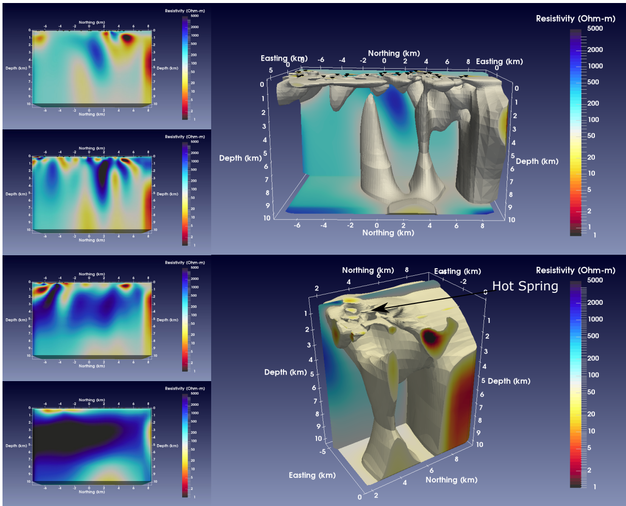
Figure 2: Different views of the resistivity model and main anomaly C1. Left: looking west through the resistivity model, where the top panel is the furthest west profile and each panel is a 3 km step west. Top Right: looking west. Bottom Right: looking northwest at the hot springs.
