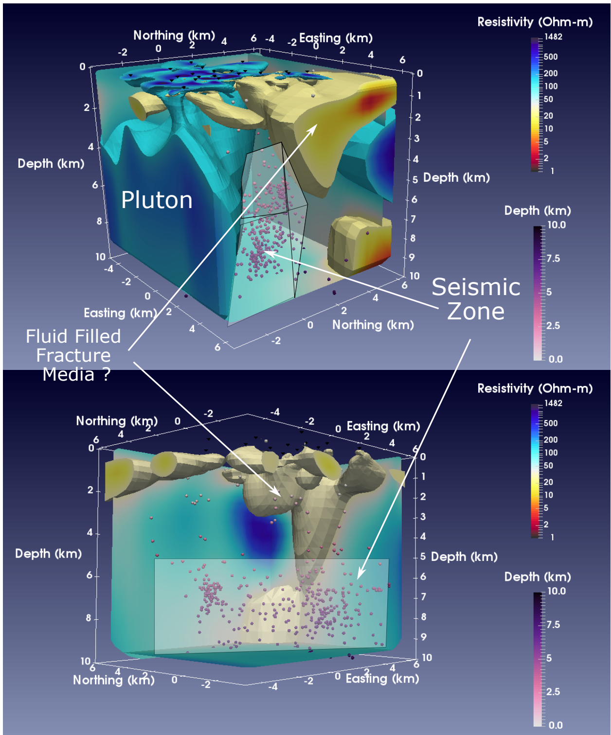
Figure 3: Views of 3-D resistivity model with preliminary interpretations.
