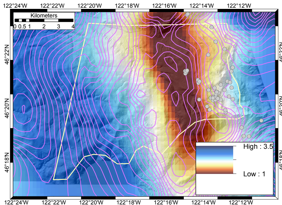
Figure 11: Resistivity depth slice at 5860 m with isostatic gravity contours (magenta lines) and earthquake locations (gray circles) within 1000 m of the depth slice.
