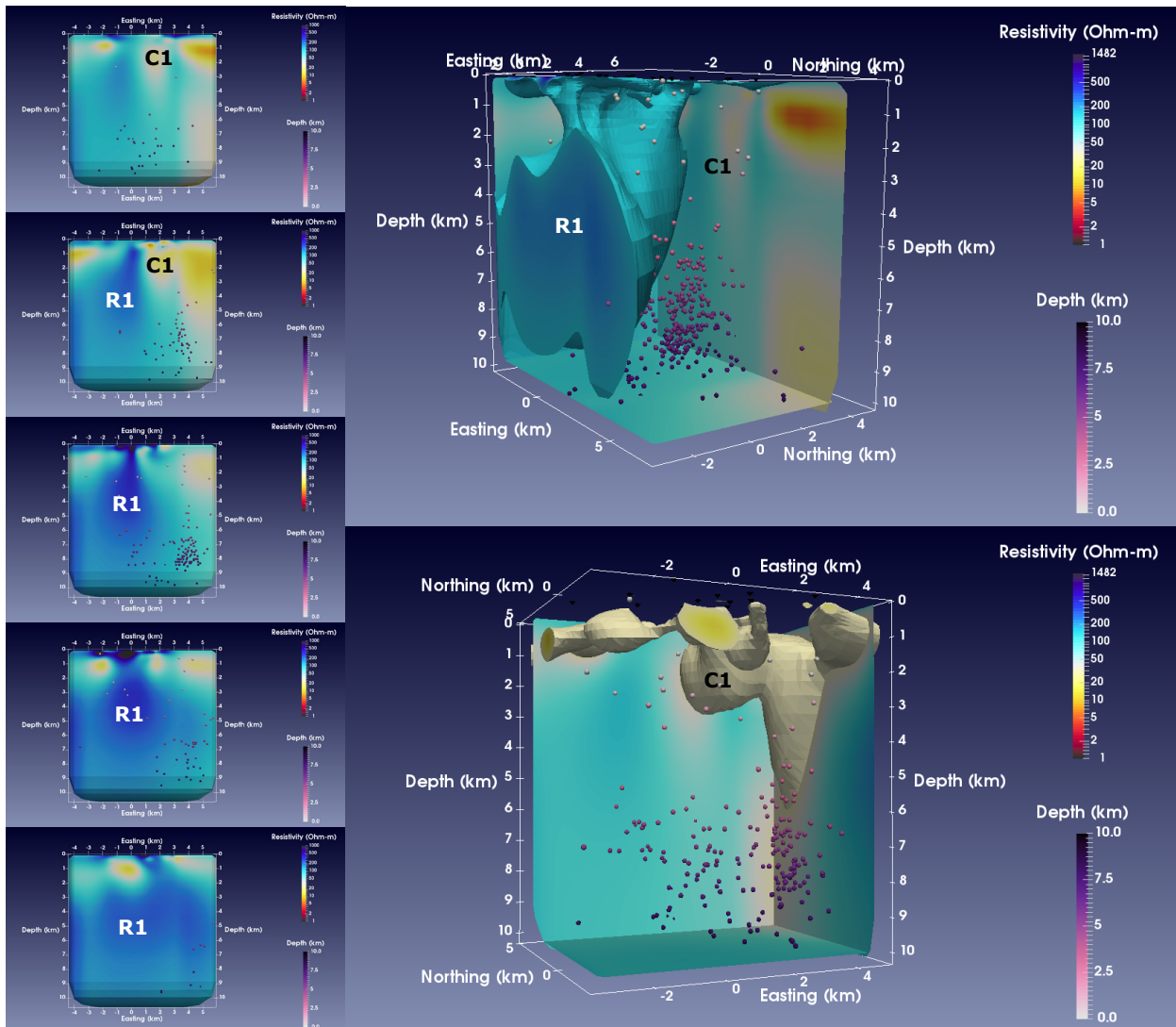
Figure 2: Different views of the resistivity model and main anomaly C1. Left: looking north through the resistivity model, where the top panel is the furthest north profile and each panel is a 1.5 km step south. . Resistivity anomalies are labeled as discussed in the text. Top Right: looking northwest at R1. Bottom Right: looking north-northeast at C1.
