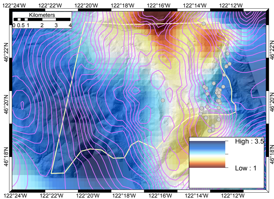
Figure 10: Resistivity depth slice at 3260 m with isostatic gravity contours (magenta lines) and earthquake locations (gray circles) within 1000 m of the depth slice.
