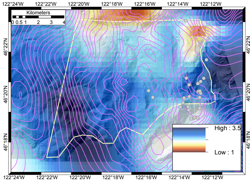
Figure 9: Resistivity depth slice at 2160 m with isostatic gravity contours (magenta lines) and earthquake locations (gray circles) within 1000 m of the depth slice.
