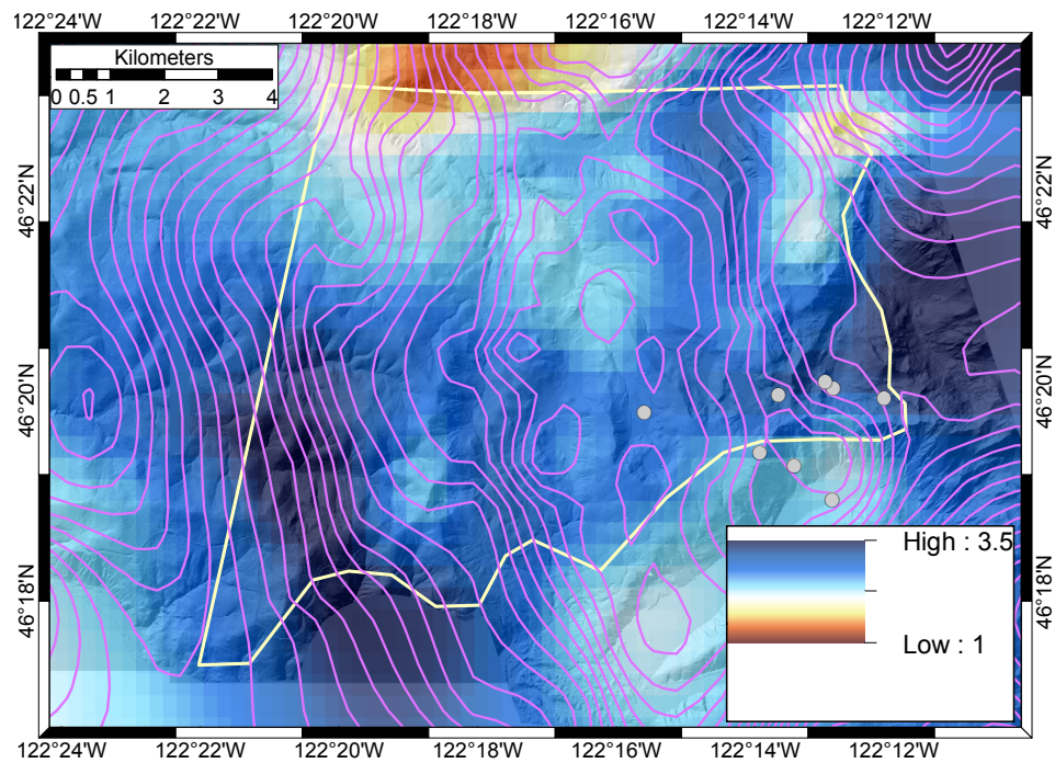
Figure 8: Resistivity depth slice at 1500 m with isostatic gravity contours (magenta lines) and earthquake locations (gray circles) within 500 m of the depth slice.
