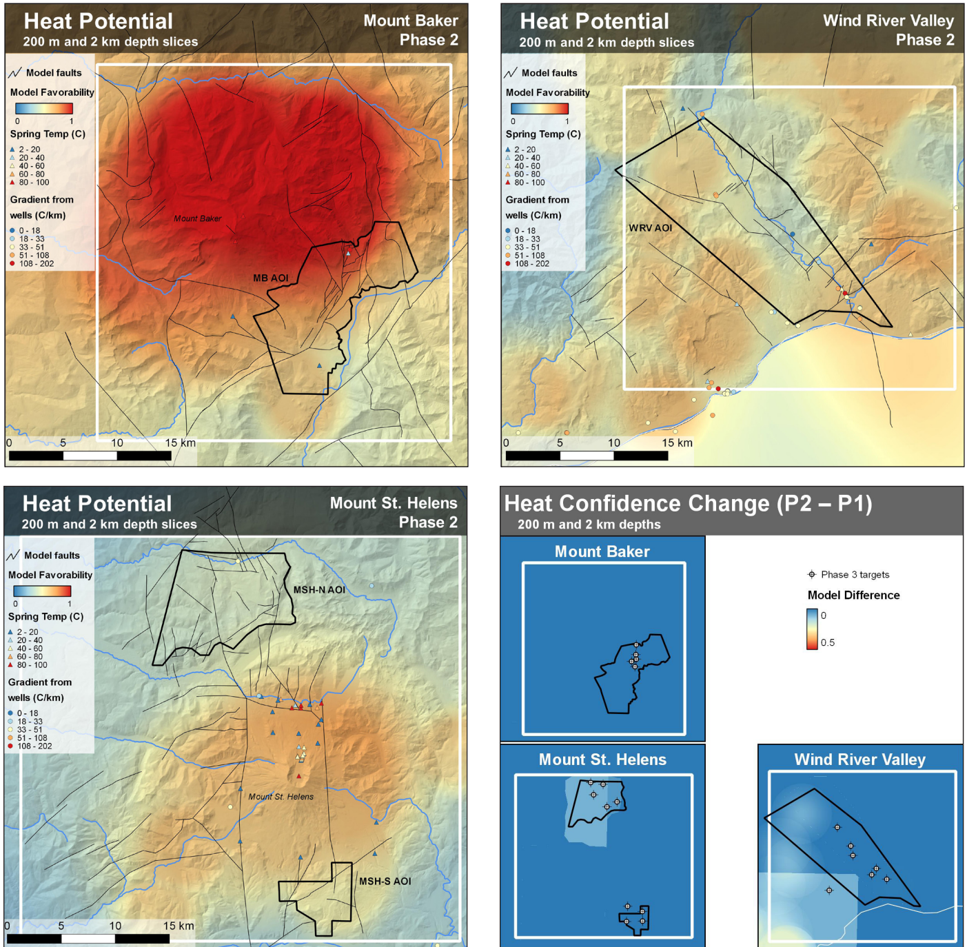
Figure 3. Phase 2 heat potential and change in confidence from Phase 1. Confidence increases are largely the result of new mapping at MSH, and opportunistic data collection near WRV. Individual confidence models are provided in Appendix J.
