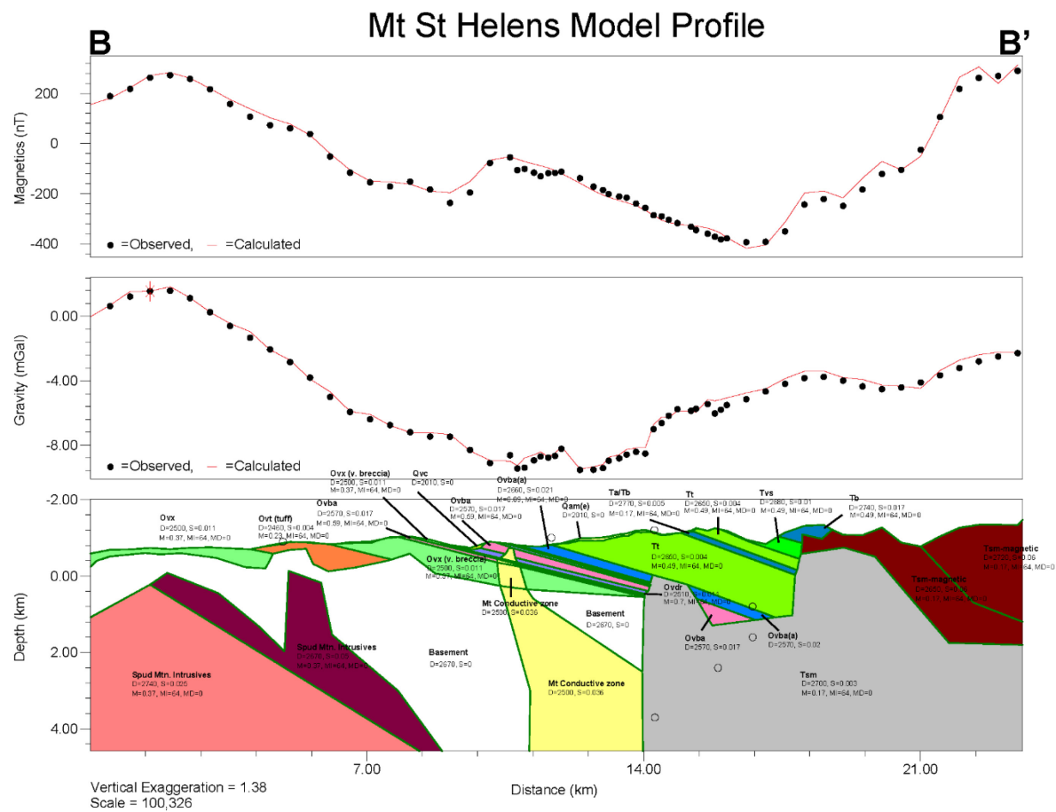
Figure 22. 2D Potential field model along profile BB' in the Mount St. Helens study area. Panels show observed (black circles) and model (red line) anomalies for magnetic (top) and gravity (middle) fields, and potential field model with individual model bodies colored by rock unit (bottom). Open circles are earthquake hypocenters from the PNSN catalog. Profile location shown in Figure 8.
