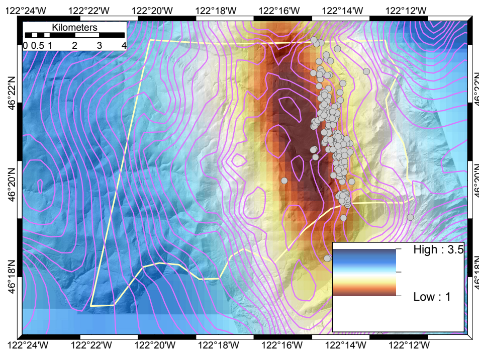
Figure 12: Resistivity depth slice at 7860 m with isostatic gravity contours (magenta lines) and earthquake locations (gray circles) within 1000 m of the depth slice.
