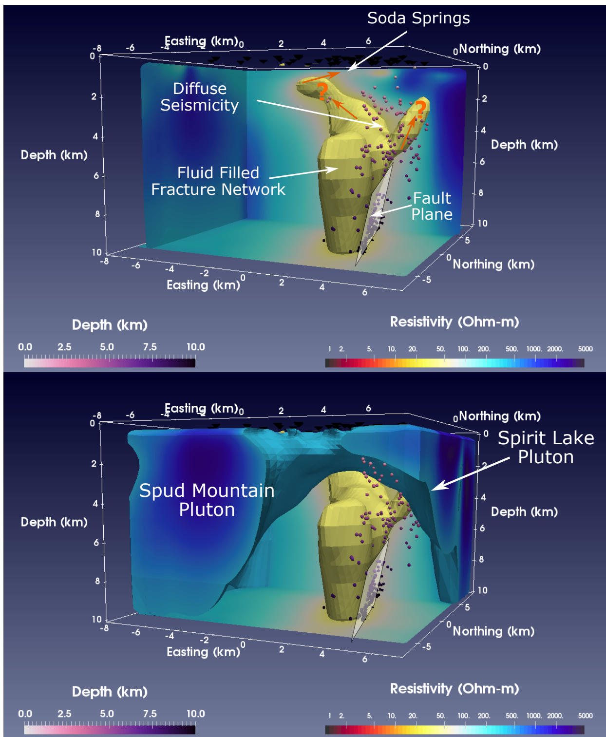
Figure 3: Views of 3-D resistivity model with preliminary interpretations. Orange arrows and question marks indicate possible fluid flow pathways and direction.
