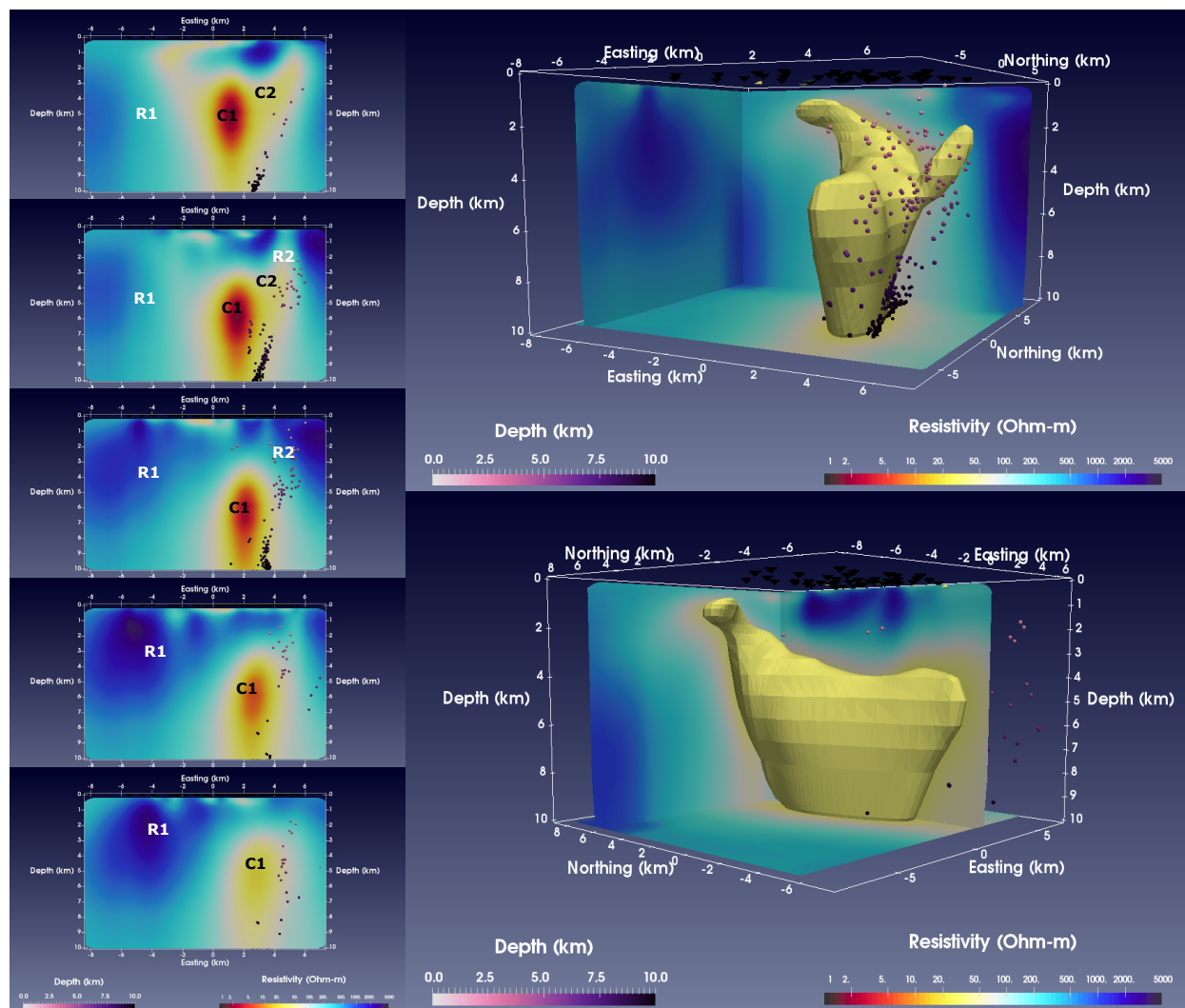
Figure 2: Different views of the resistivity model and main anomaly C1. Left: looking north through the resistivity model each panel is a 2 km step north. Resistivity anomalies are labeled as discussed in the text. Top Right: looking northeast at the C1. Bottom Right: looking north-northwest along C1.
