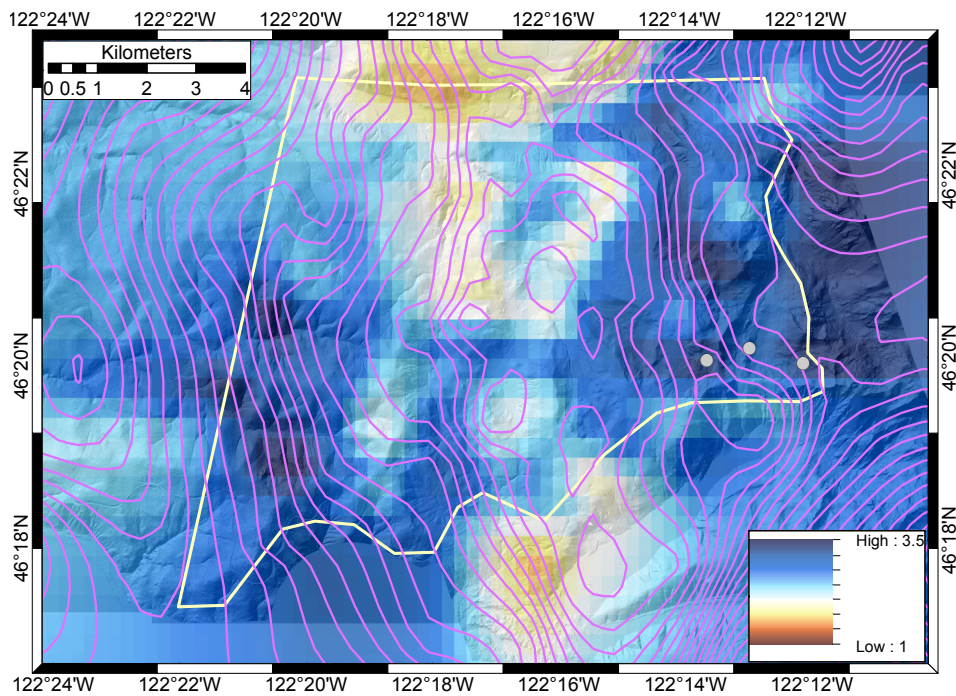
Figure 6: Resistivity depth slice at 560 m with isostatic gravity contours (magenta lines) and earthquake locations (gray circles) within 200 m of the depth slice.
