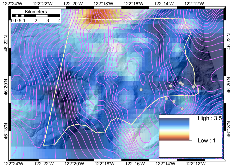
Figure 7: Resistivity depth slice at 960 m with isostatic gravity contours (magenta lines) and earthquake locations (gray circles) within 300 m of the depth slice.
