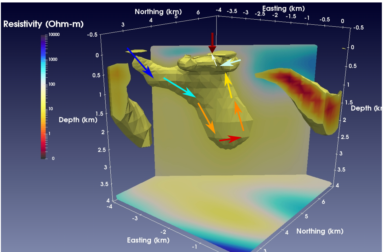
Figure 3: A closer look at the conductive anomaly associated with the Baker Hot Springs. The view is looking to the east northeast. The red arrow at the surface mark the location of the hot spring. The threshold on the resistivity is 10 Ohm-m. The thought is that cold meteoric water seeps down through deep faults to a depth of around 3 km (cool colored arrows), then heats up (red arrows) and up flows to the Baker Hot Spring while mixing with near surface meteoric water.
