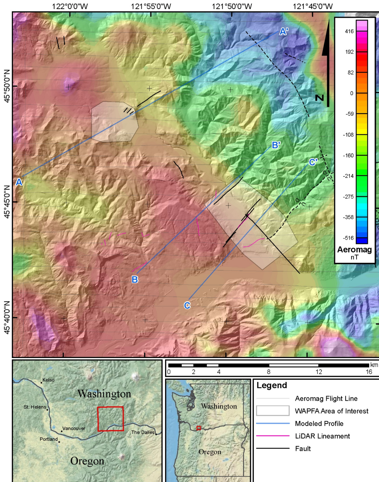
Figure 3. Reduced to Pole, Residual Aeromagnetic data flown in 1982. Flight lines included. (U.S Geological Survey, 1982)
