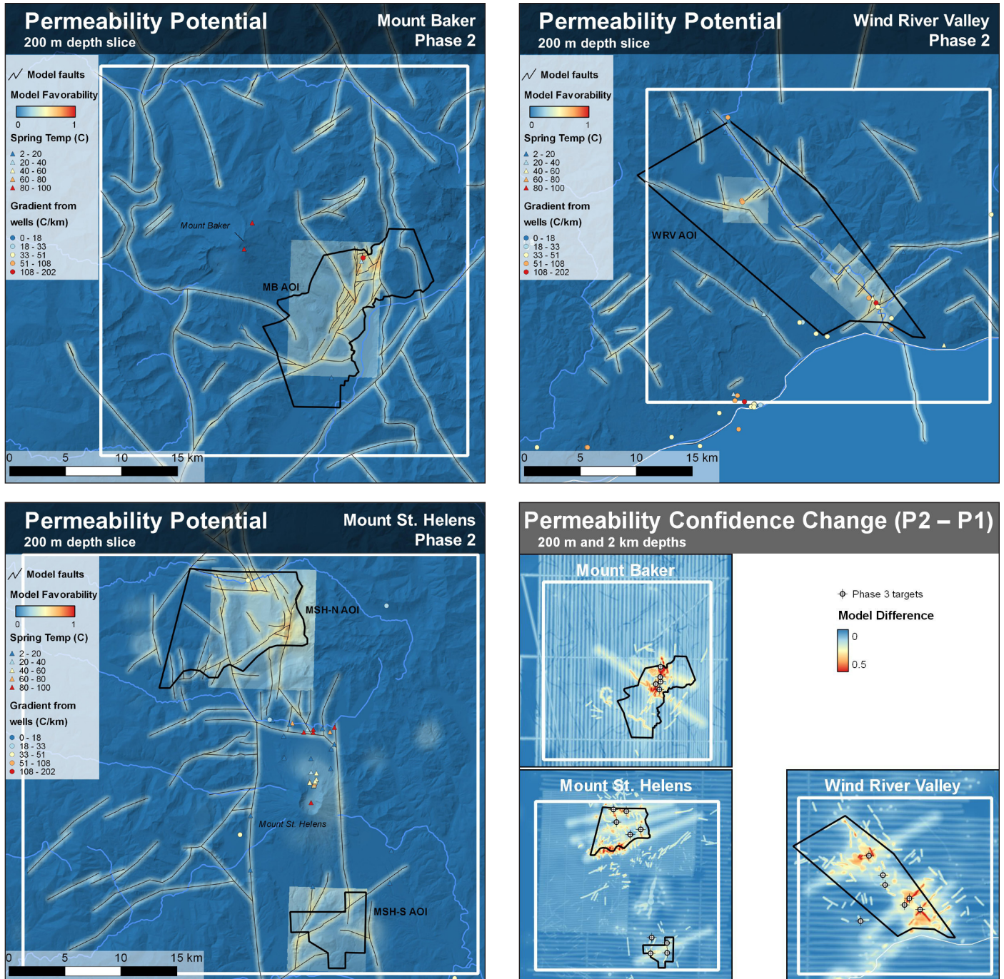
Figure 4. Phase 2 permeability potential at 200 m depth and change in confidence from Phase 1. Confidence increases are the result of new mapping, lidar interpretation, the inclusion of new gravity and magnetic data, modeled cross sections, and updated and refined geomechanical models and opportunistic data collection near WRV. Potential models at 2 km depth are provided in Appendix I and confidence models are provided in Appendix J.
