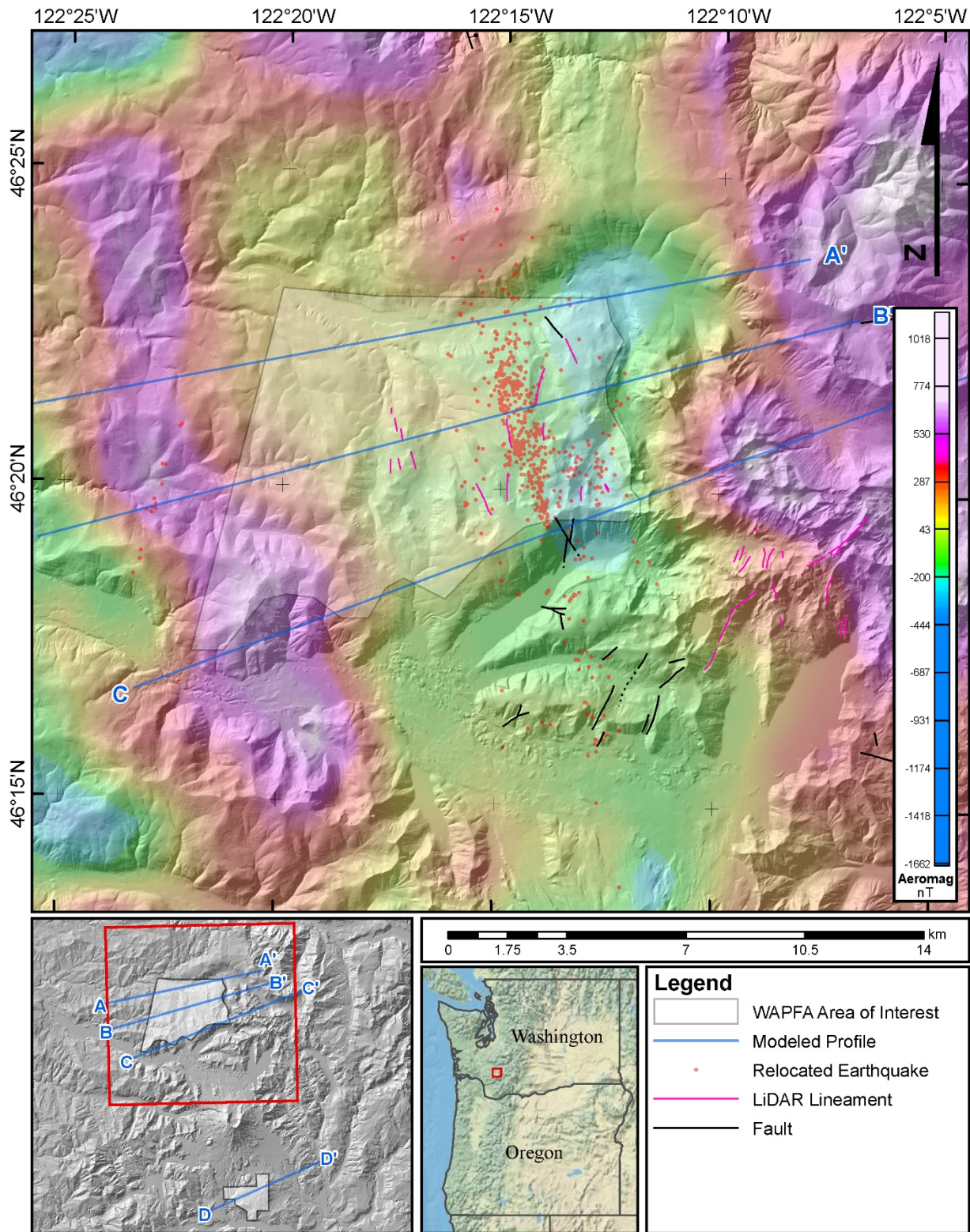
Figure 13. Reduced to Pole, Residual Aeromagnetic data within the Northern Area of Interest (Blakely et al. 2016).
