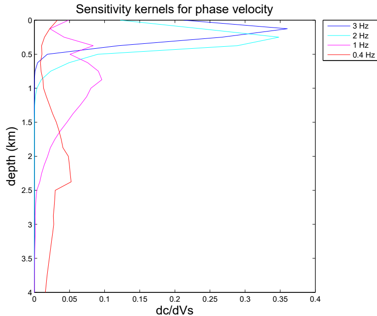
Figure 7. Sensitivity kernel for each of the frequencies used. Shows how deep the structure of the phase velocity is sensitive to.
