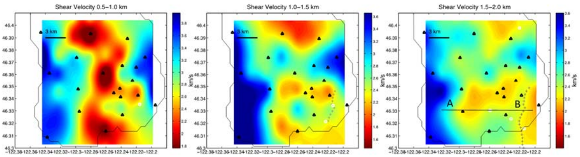
Figure 9. Shear velocity maps for shallow depth slices (see titles). Seismicity white circles, mapped faults grey crosses. Line where A-B transect is projected (Figure 11) is on right plot. The black contour outlines where the resolution matrix was nonzero in the most resolved phase velocity map.
