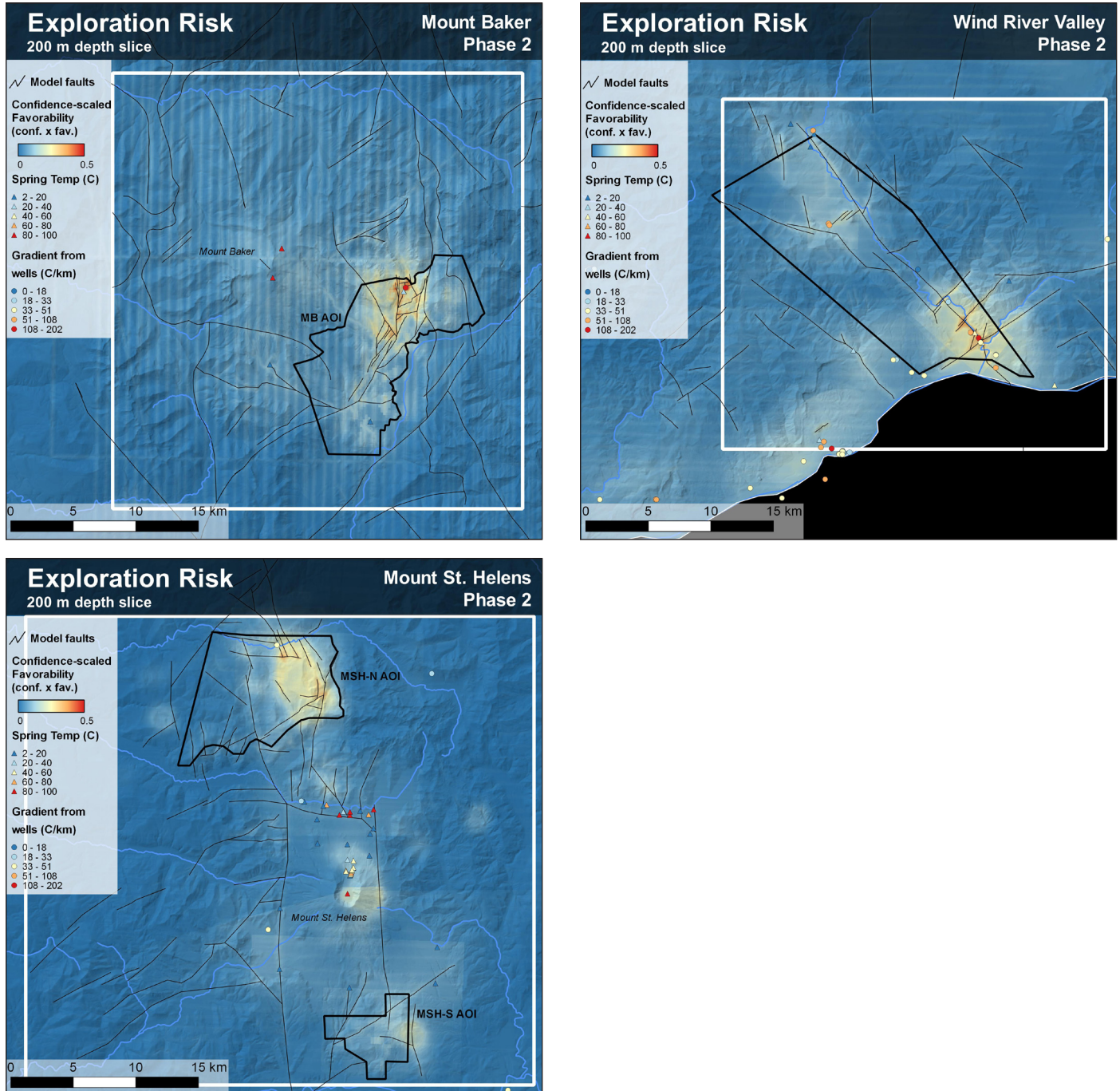
Figure 8. Exploration 'risk' models for all three study areas at 200 m depth.
