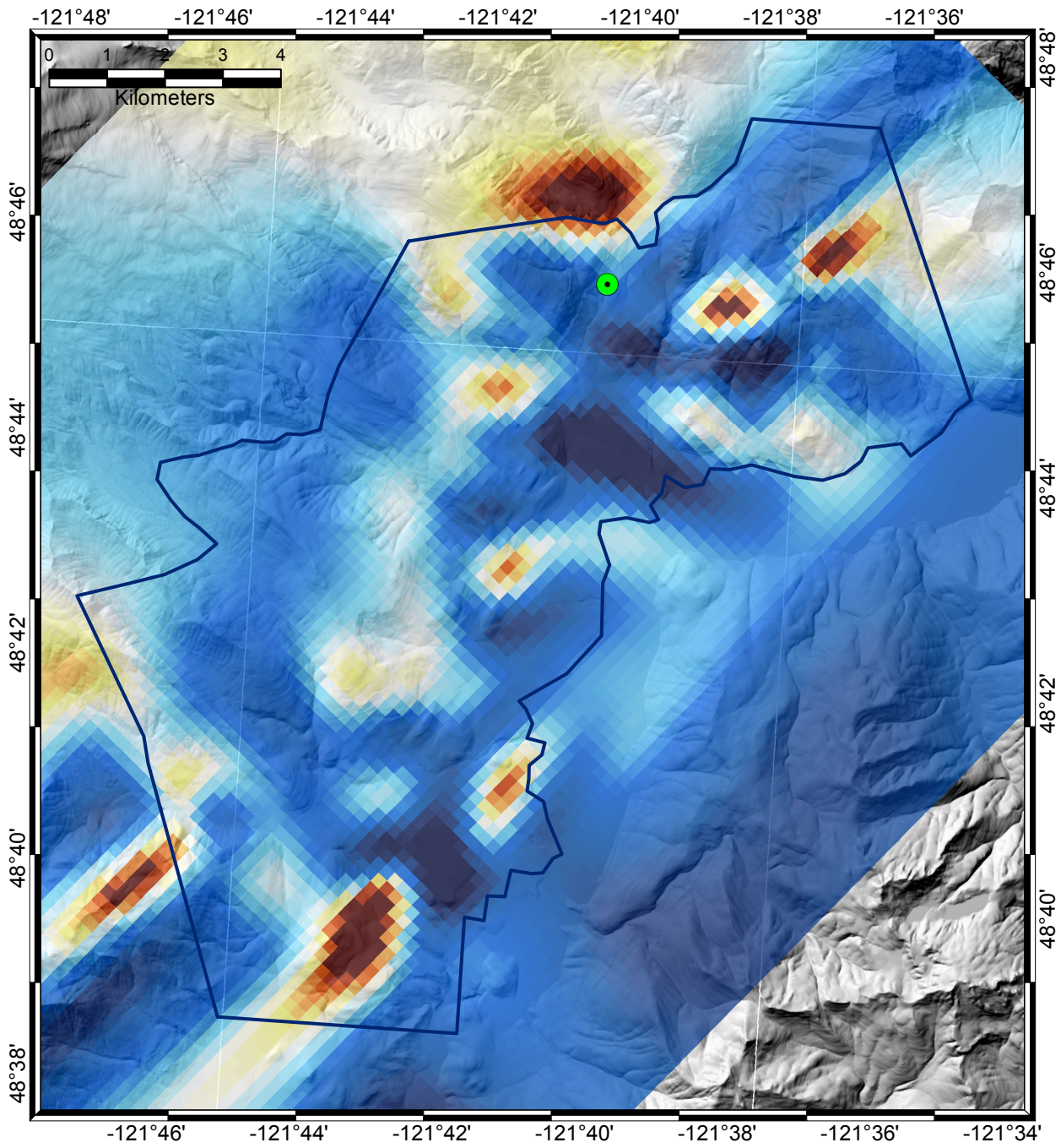
Figure 6: Depth slice at 960 m. Green dot is hot spring location.
